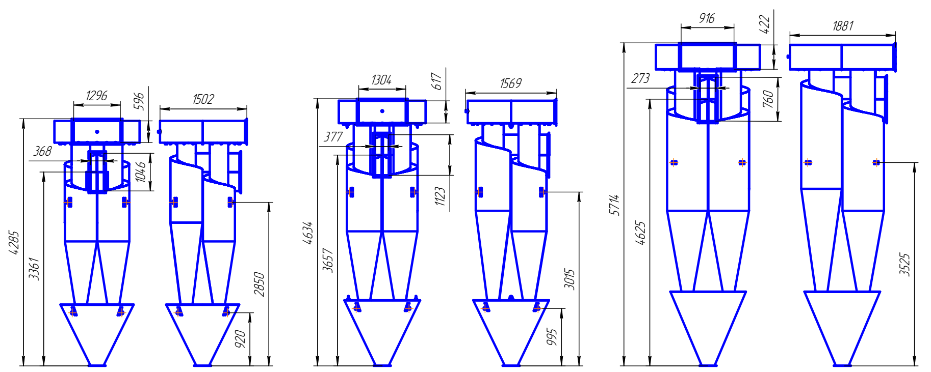
ЦБ-4-225 ЦБ-4-250 ЦБ-4-275 ЦБ-4-300 ЦБ-4-350
