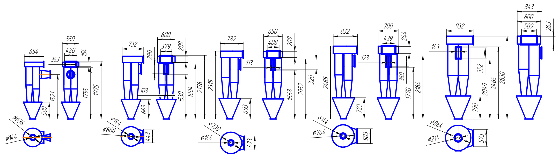
ЦБ-4-225 ЦБ-4-250 ЦБ-4-275 ЦБ-4-300 ЦБ-4-350
